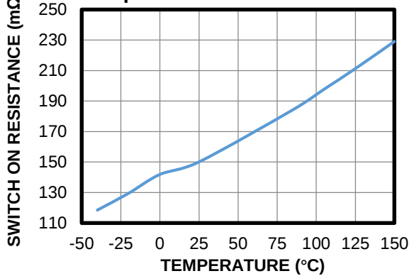
Switch On Resistance vs. Temperature
