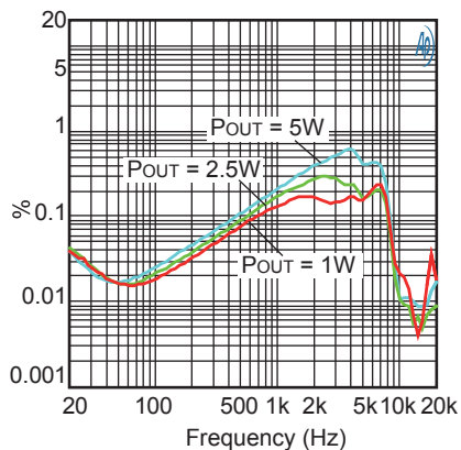
THD+N vs. Frequency (12V, 4Ω+33μH)
