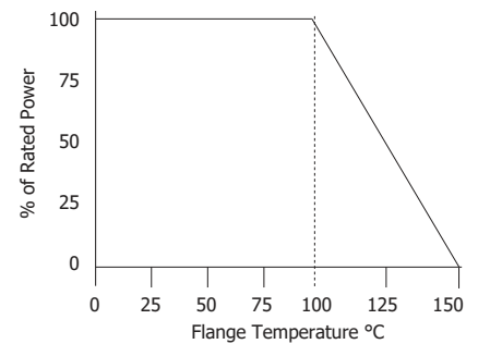
AA0600-250-17X Power Derating Curve
