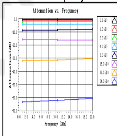
Attenuation vs. Frequency
