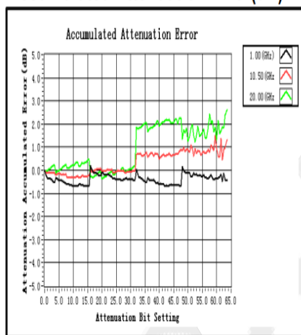
Accumulated Attenuation Error (dB)
