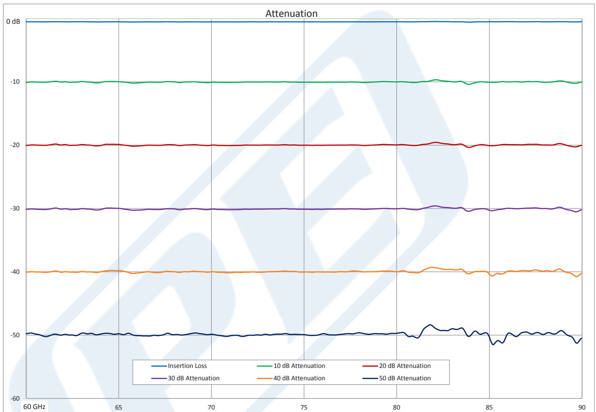
Typical Performance Data
