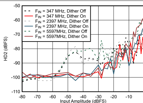
Figure 6-72. Dual Channel Mode: HD2 vs Input Amplitude and Dither
