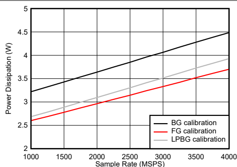
Figure 6-132. Dual Channel Mode: Power Dissipation vs Sample Rate
