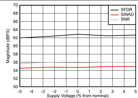
Figure 6-102. Dual Channel Mode: SNR, SINAD and SFDR vs Supply Voltage
