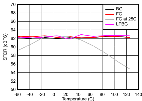
Figure 6-97. DES Mode: SFDR vs Temperature and Calibration Mode
