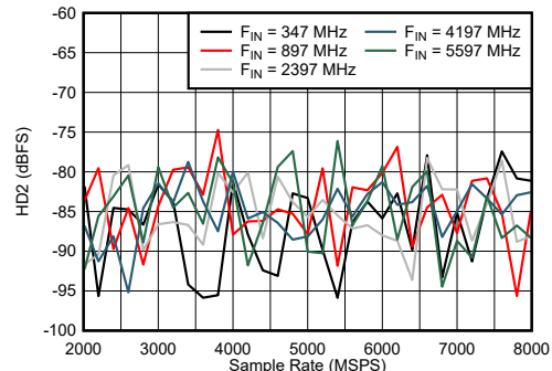
Figure 6-34. DES Mode: HD2 vs Sample Rate and Input Frequency
