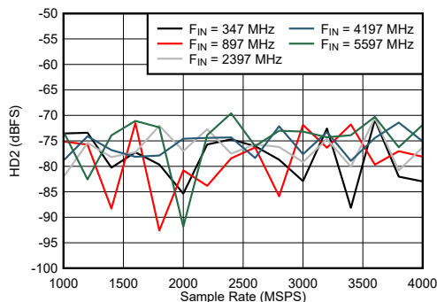
Figure 6-49. Dual Channel Mode: HD2 vs Sample Rate and Input Frequency
