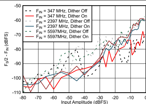
Figure 6-64. DES Mode: F_{\text{S}}/2 - F_{\text{IN}} vs Input Amplitude and Dither
