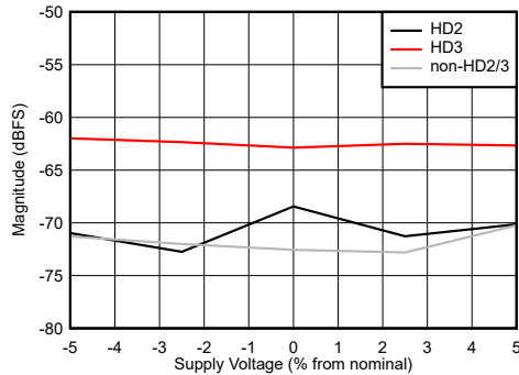
Figure 6-103. Dual Channel Mode: HD2, HD3 and Worst non-HD Spur vs Supply Voltage
