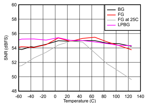
Figure 6-94. Dual Channel Mode: SNR, SINAD and SFDR vs Temperature
