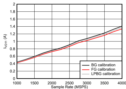
Figure 6-119. DES Mode: I_{VD11} vs Sample Rate
