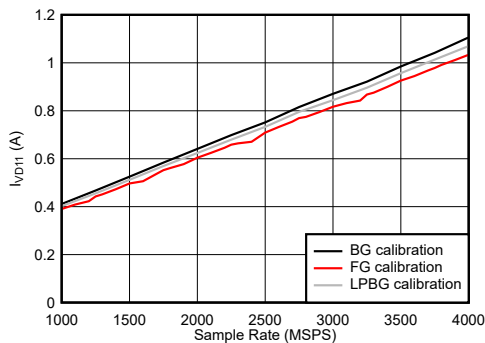
Figure 6-118. DES Mode: I_{VD11} vs Sample Rate
