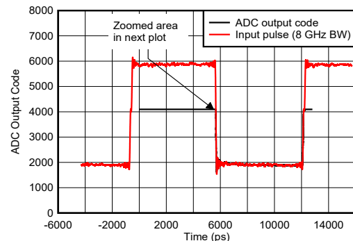
Figure 6-141. Pulse Overdrive Recovery
