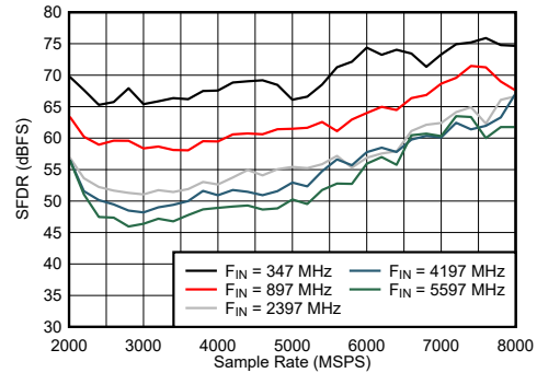
Figure 6-32. DES Mode: SFDR vs Sample Rate and Input Frequency
