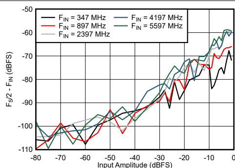
Figure 6-63. DES Mode: F_{\text{S}}/2 - F_{\text{IN}} vs Input Amplitude and Frequency
