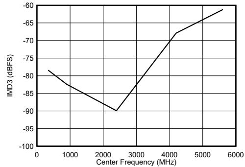
Figure 6-104. DES Mode: IMD3 vs Input Frequency
