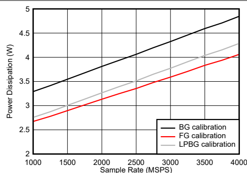
Figure 6-133. Dual Channel Mode: Power Dissipation vs Sample Rate
