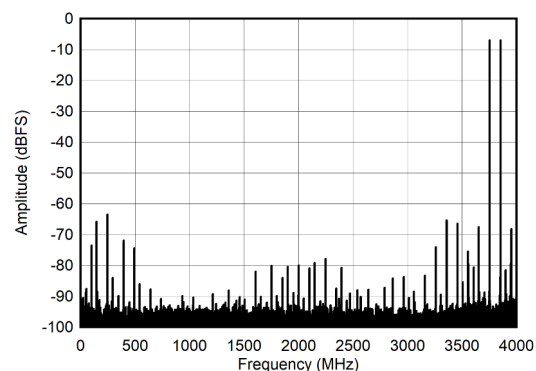
Figure 6-16. DES Mode: Two Tone FFT at 4197 MHz
