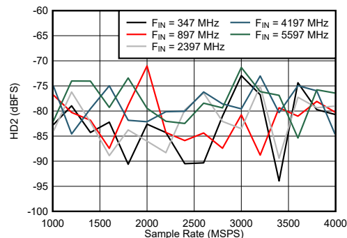
Figure 6-50. Dual Channel Mode: HD2 vs Sample Rate and Input Frequency
