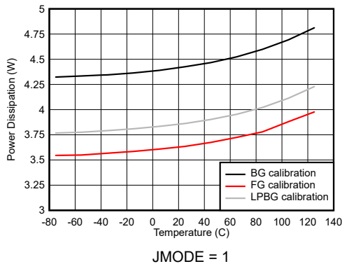
Figure 6-136. DES Mode: Power Dissipation vs Temperature
