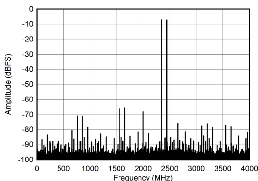
Figure 6-15. DES Mode: Two Tone FFT at 2397 MHz
