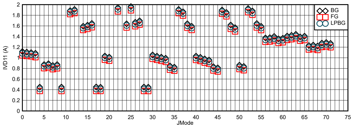
Figure 6-115. I_{V_{D11}} vs JMODE at F_{\text{CLK}} = 4\text{ GHz}
