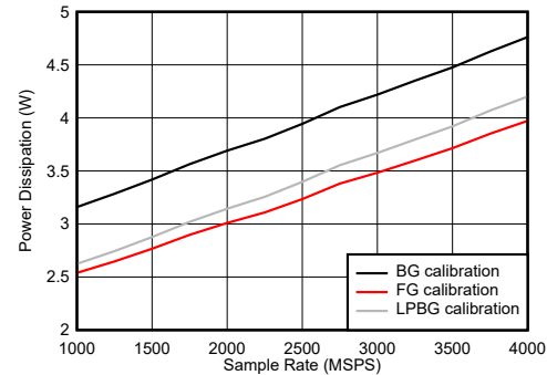
Figure 6-125. DES Mode: Power Dissipation vs Sample Rate
