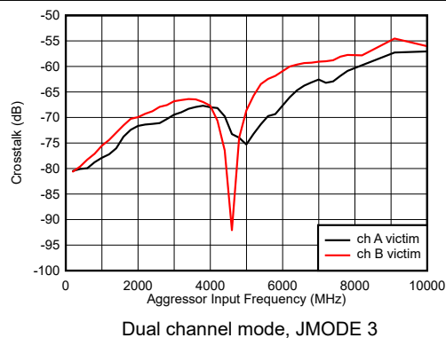
Figure 6-5. Crosstalk vs Input Frequency
