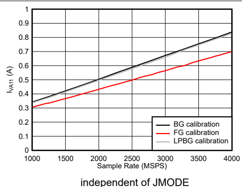
Figure 6-117. DES Mode: I_{V_{A11}} vs Sample Rate
