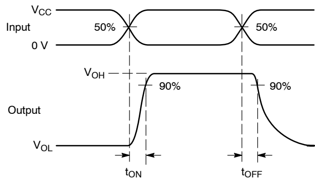
Figure 3. t_{ON}/t_{OFF}
