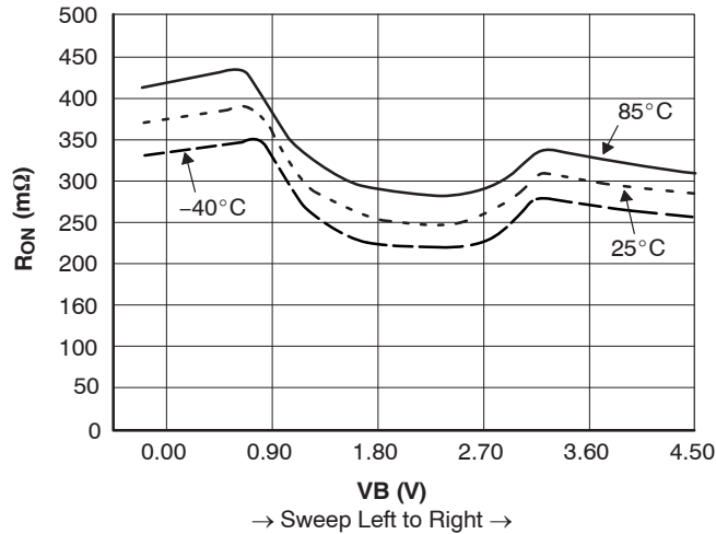
Figure 5. R_{ON} Switch On Resistance, I_{ON} = 100 mA, V_{CC} = 4.3 V B0
