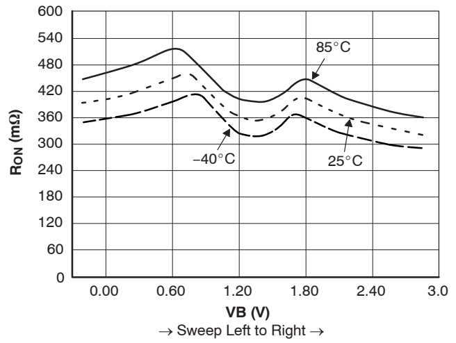
Figure 6. R_{ON} Switch On Resistance, I_{ON} = 100 mA, V_{CC} = 2.7 V B0
