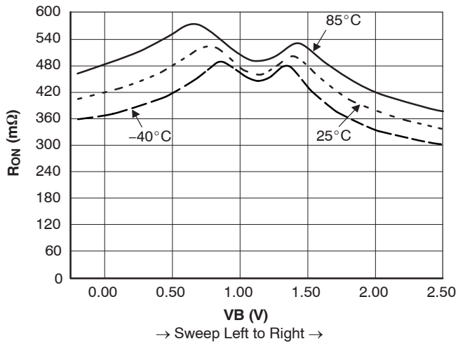
Figure 4. R_{ON} Switch On Resistance, I_{ON} = 100 mA, V_{CC} = 2.3 V B0
