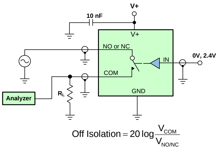
Figure 4 — Off-Isolation
