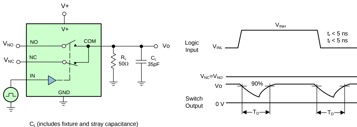
Figure 2 — Break-Before-Make Interval
