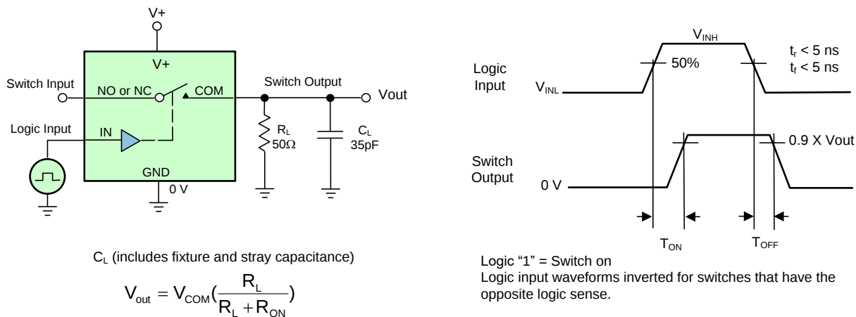
Figure 1 — Switching Time
