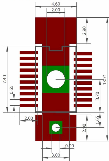
TSSOP-20 LAND PATTERN All dimensions are in millimeters
