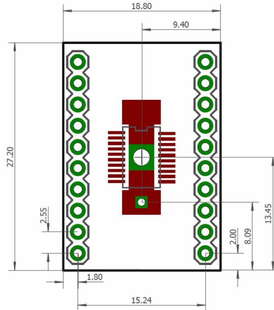
TSSOP-20 BOARD SIZE All dimensions are in millimeters
