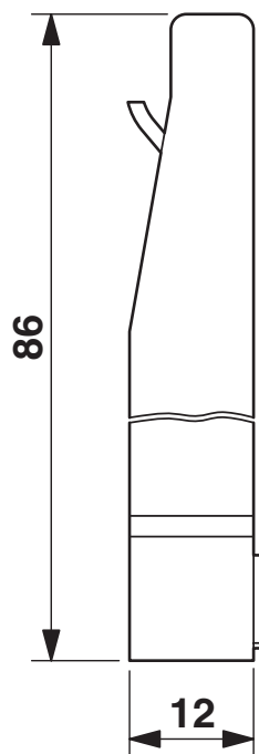
Dimensional drawing
