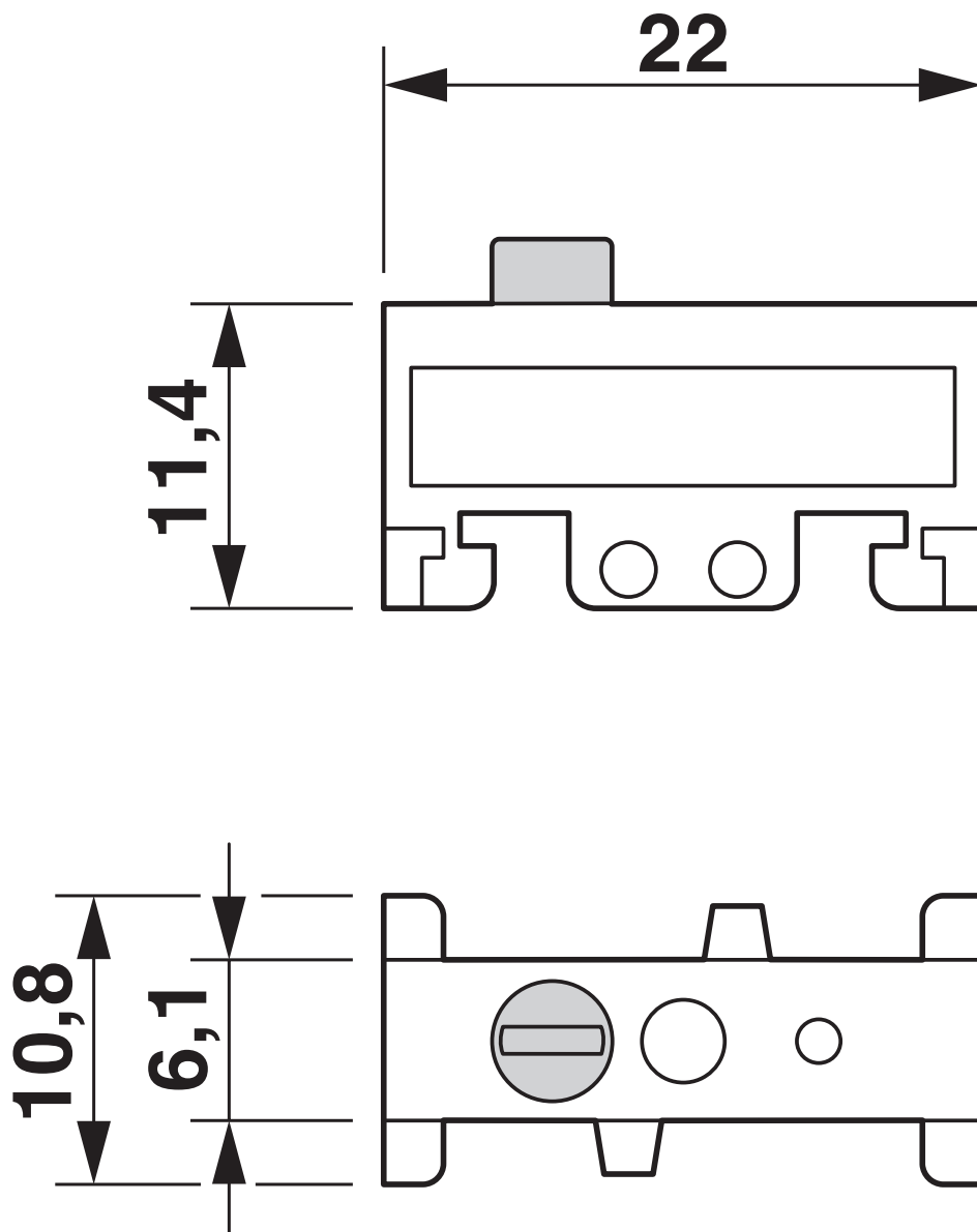
Dimensional drawing
