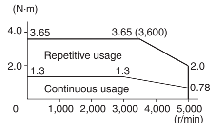
R88M-GP40030H/T (400 W)
