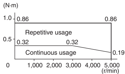
R88M-GP10030H/T (100 W)
