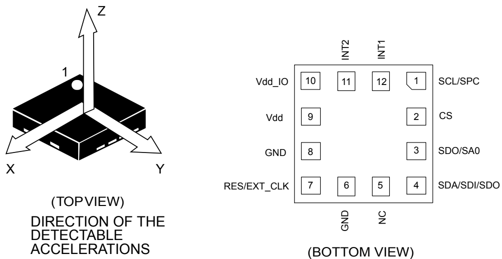
Figure 2. Pin connections
