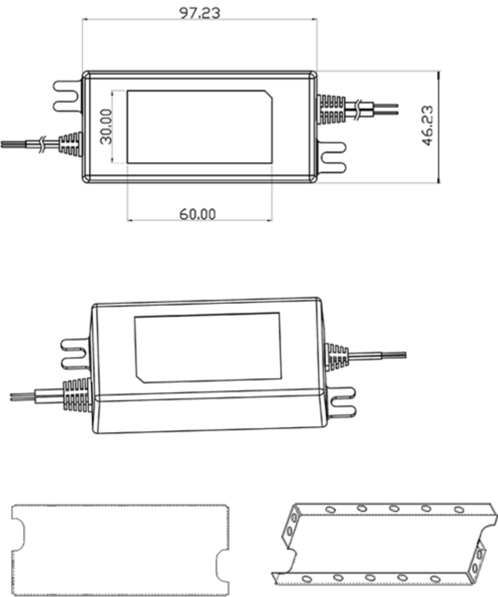
MYLAR CASE COVER INSTALLED
