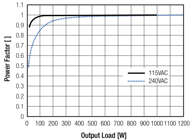
Power Factor
