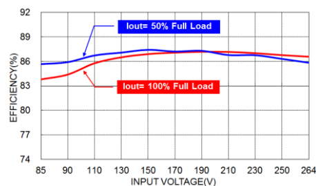
MAC15US12D Efficiency vs. Input Voltage
