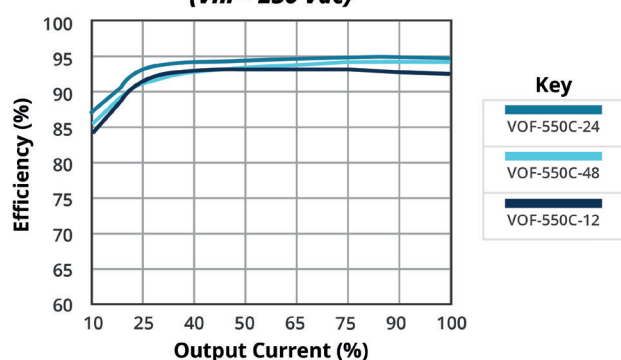
EFFICIENCY VS OUTPUT LOAD ( V_{in} = 230 \text{ Vac} )
