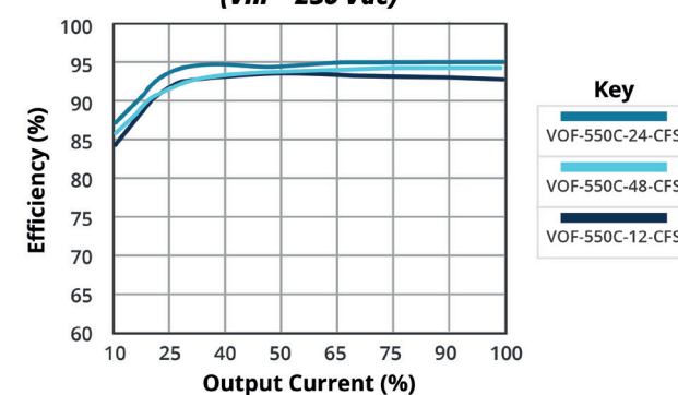
EFFICIENCY VS OUTPUT LOAD ( V_{in} = 230 \text{ Vac} )
