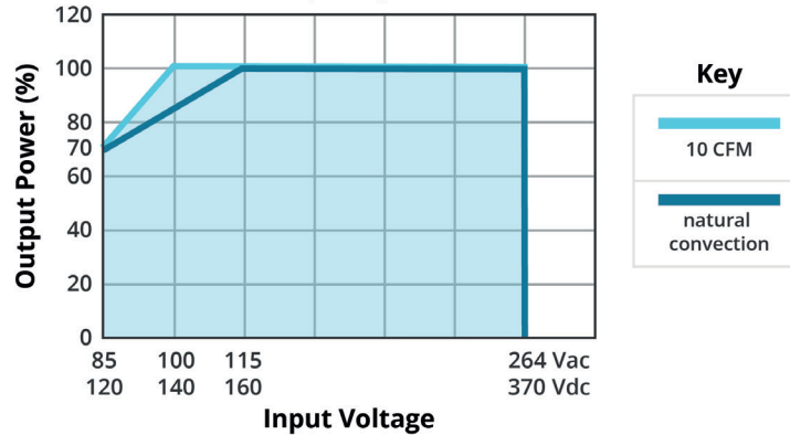
INPUT VOLTAGE DERATING CURVE (25°C)
