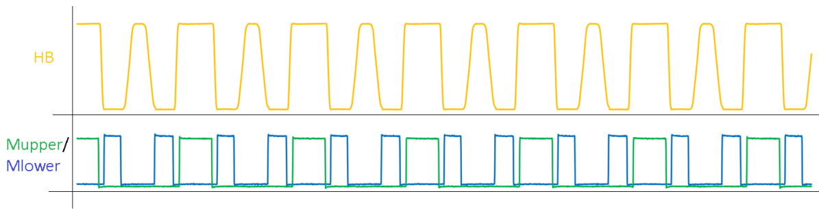
Figure 49. Light-load Operation
