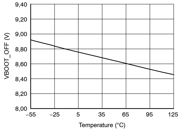
Figure 11. V_{BOOT\_OFF} vs. Temperature
