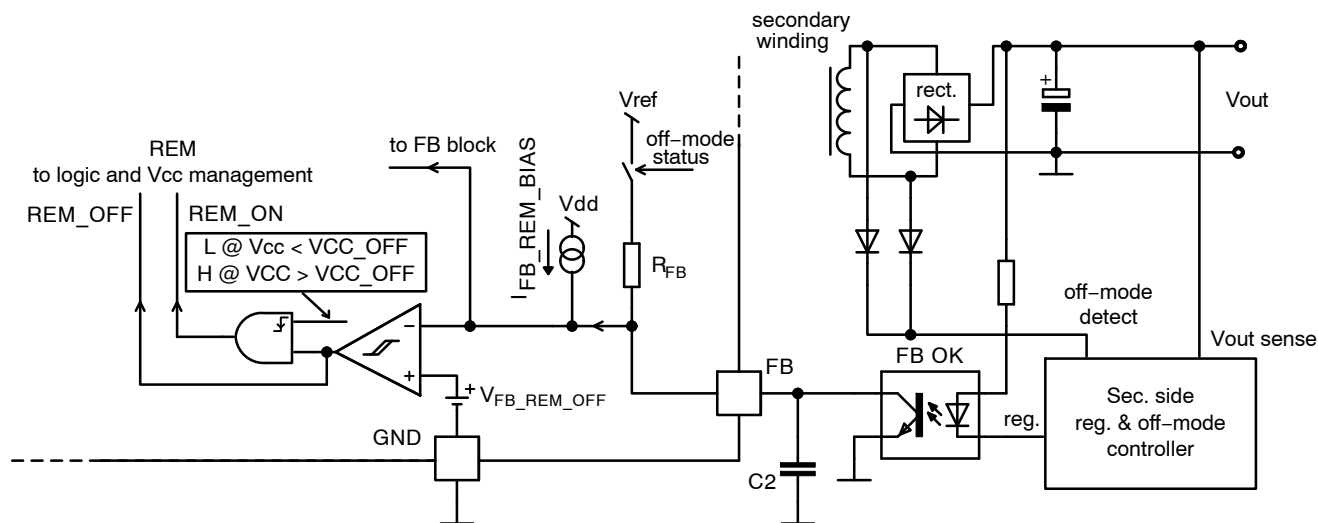
Figure 35. Active OFF Off-mode Internal Detection Based on the LLC FB Pin Voltage
