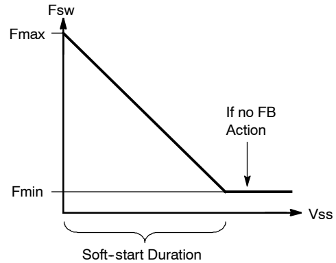
Figure 41. Soft-start Behavior
