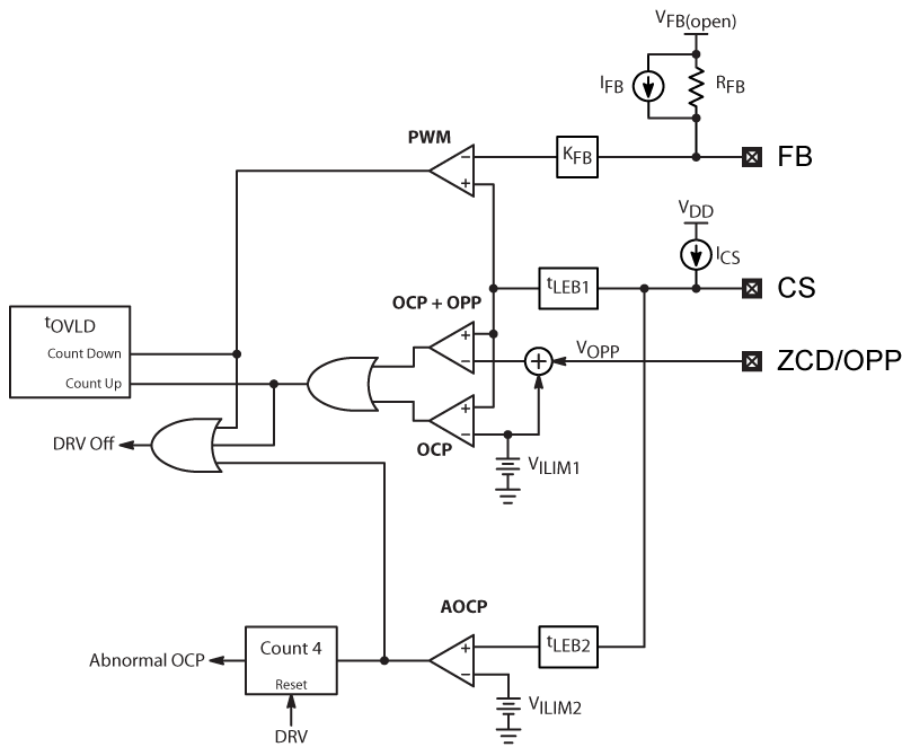
Figure 32. Overload Circuitry
