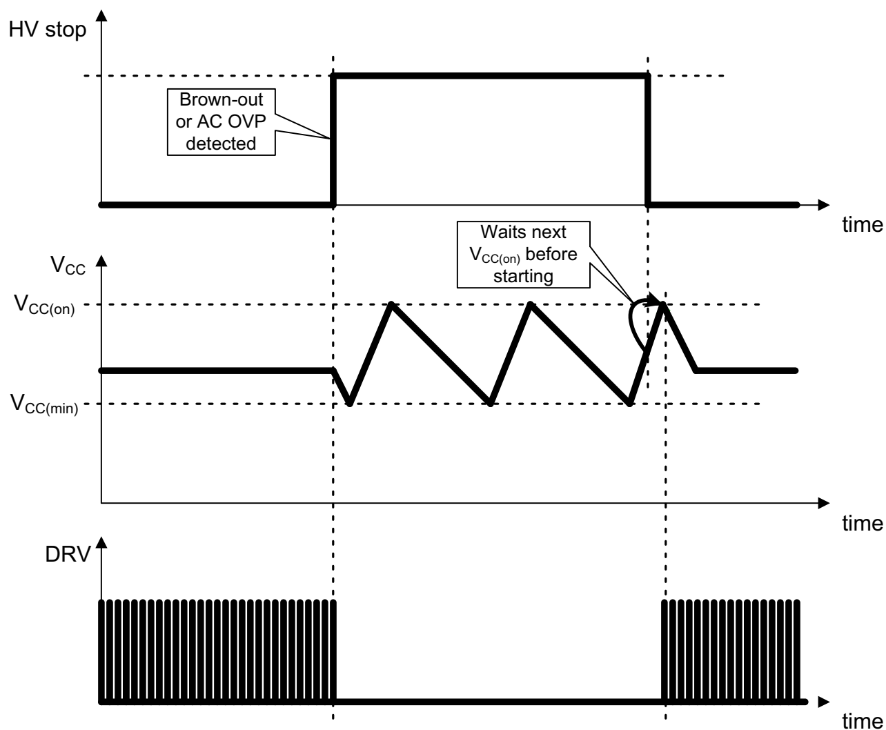
Figure 43. Brown-out or Line Overvoltage Timing Diagram
