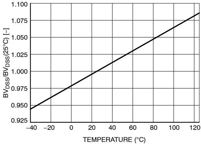
Figure 31. BV DSS /BV DSS (25°C) vs. Temperature
