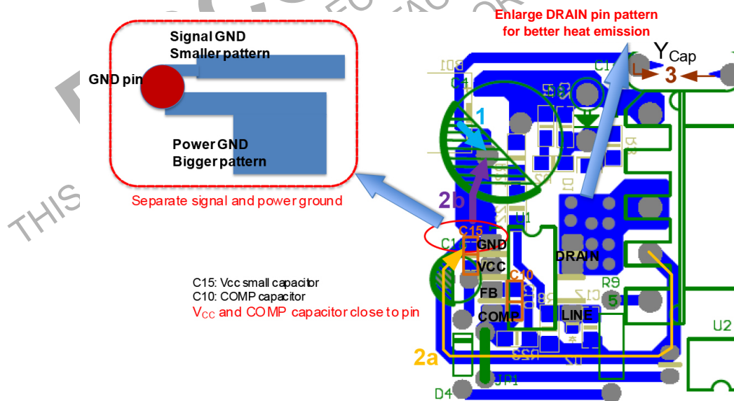
Figure 48. Layout Considerations
