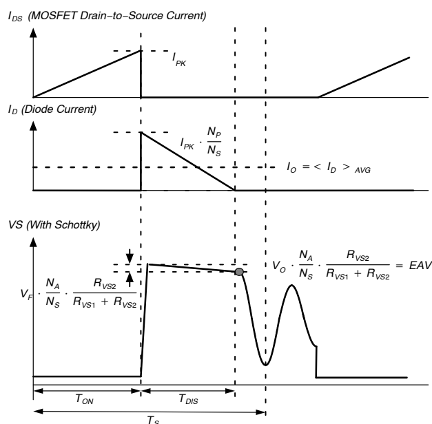
Figure 25. Cycling Current and VS Sampling in DCM
