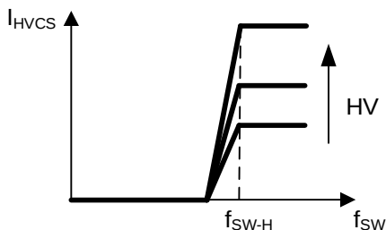
Figure 6: Current on the CS Pin for Line Compensation
