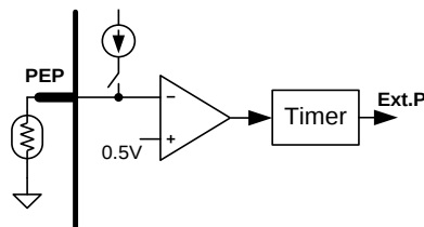
Figure 7: Primary External Protection
