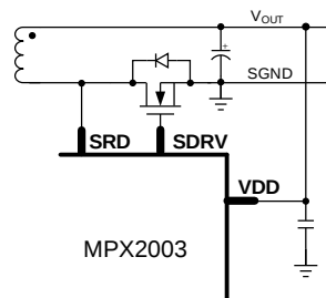
Figure 8: V_{DD} Supply from the Output
