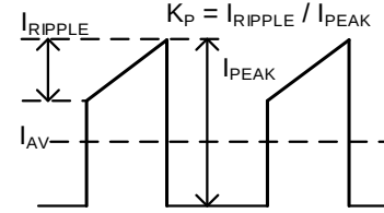
Figure 14: Typical Primary Current Waveform
