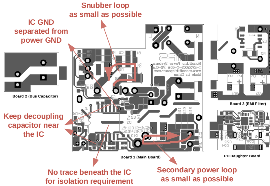
Figure 24: Recommended PCB Layout for 65W PD Adapter Design (Bottom Side)
