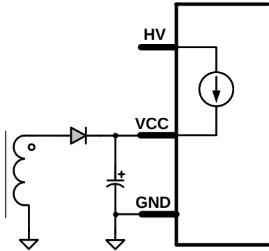
Figure 13: Start-Up Circuit
