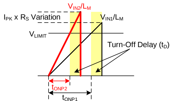
Figure 4: Peak Current Difference Caused by Turn-Off Delay
