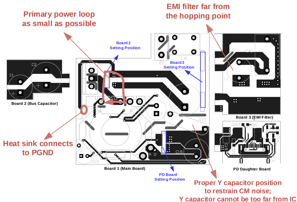
Figure 23: Recommended PCB Layout for 65W PD Adapter Design (Top Side)
