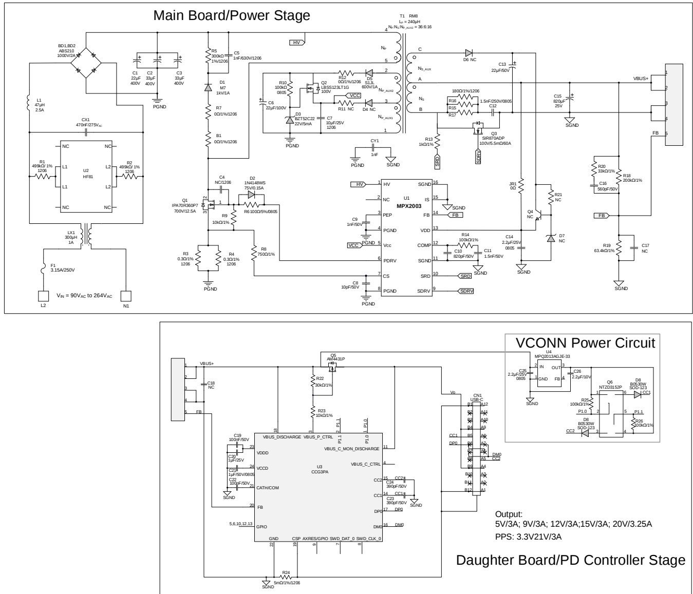
Figure 25: Example of the 65W PD Typical Application
