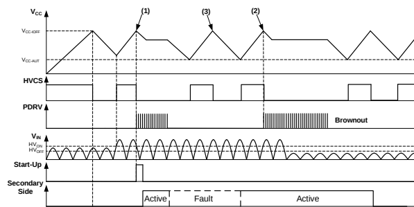
Figure 2: Start-Up Logic for the Primary IC
