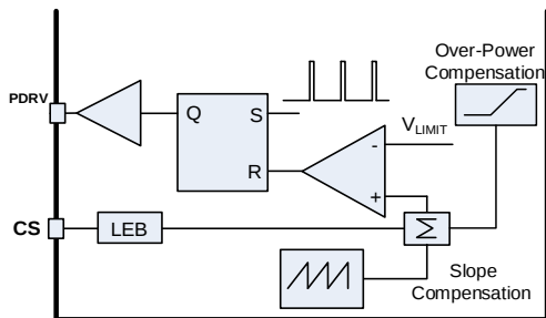
Figure 15: Peak Current Comparator Circuit Logic
