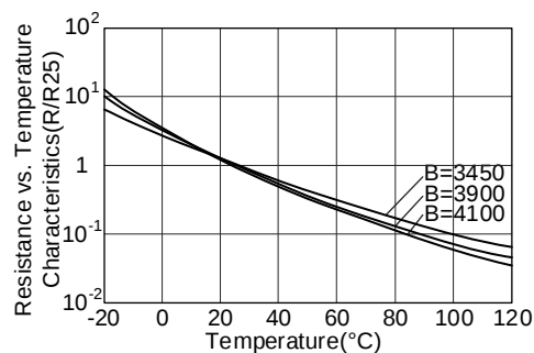
Figure 19: NTC Resistance vs. Temperature
