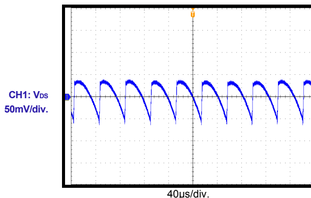
Output Ripple
