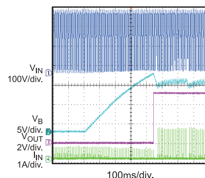
VB Short to GND Protection Recovery
