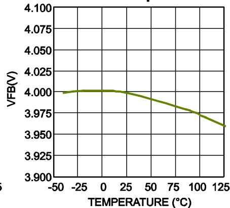
Feedback Threshold vs. Junction Temperature
