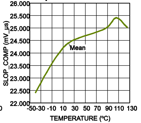
Slop_Comp vs. Temperature
