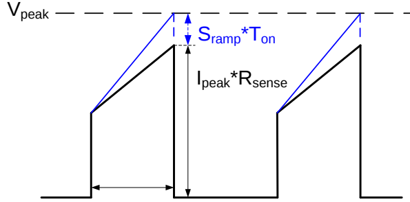
b) Typical Waveform
