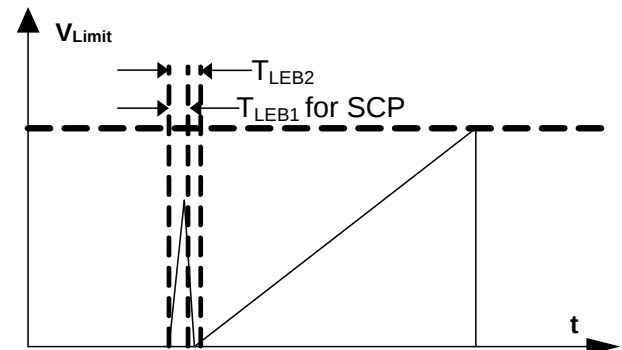
Figure 10: Leading-Edge Blanking
