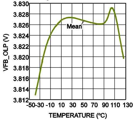
VFB_OLP vs. Temperature
