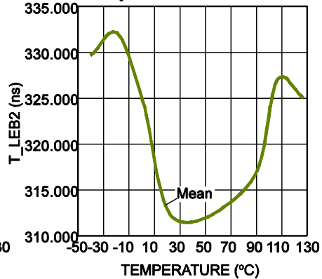
T_LEB2_LOW vs. Temperature
