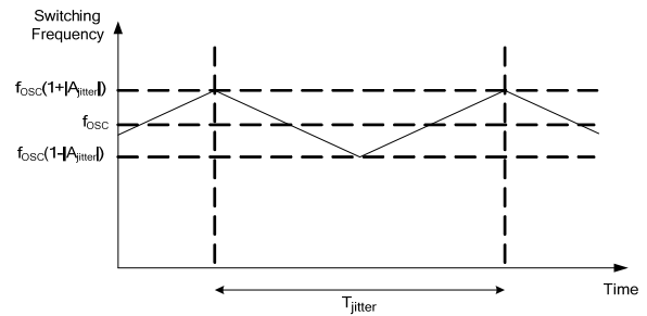
Figure 3: Frequency Jittering
