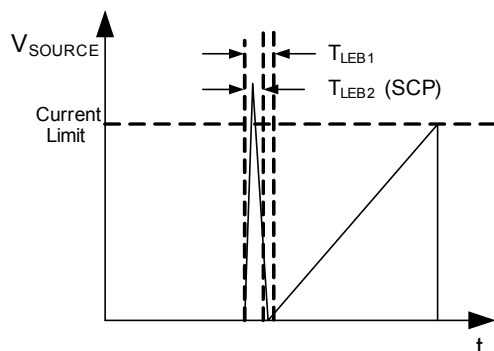
Figure 10: Leading-Edge Blanking
