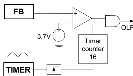
Figure 7: Overload Protection Block
