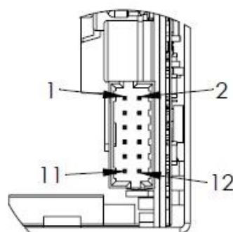
DETAIL L
