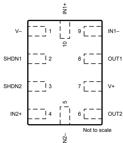
Figure 5-7. TLV9102S RUG Package 10-Pin X2QFN Top View
