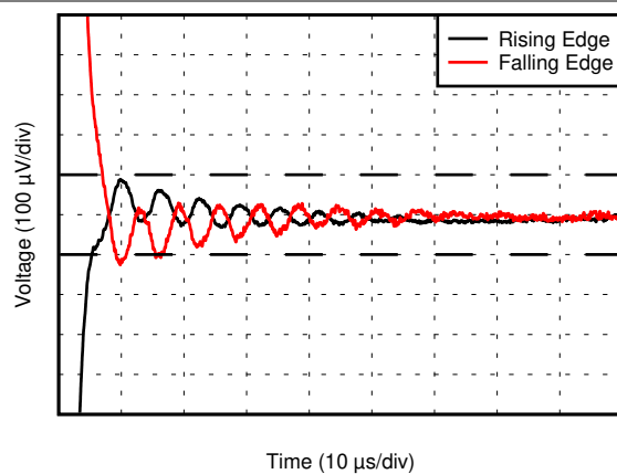
Figure 5-26. Settling Time
