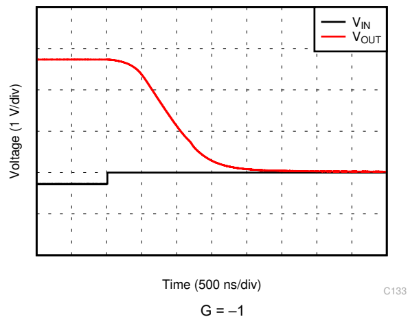
Figure 5-23. Overload Recovery
