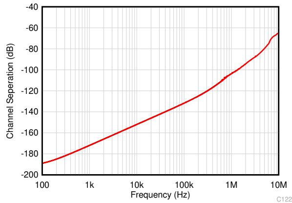
Figure 5-13. Channel-to-Channel Crosstalk
