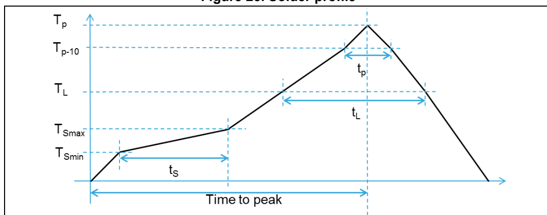
Figure 23. Solder profile
