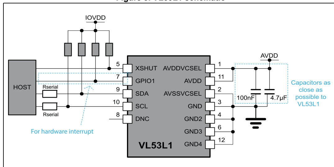
Figure 3. VL53L1 schematic
