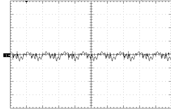
Figure 8. Output Voltage Ripple (50mV/div), time scale - 2uS/div. Vin=Vin_nom, full resistive Cout=1uF ceramic + 47uF Ceramic (see Fig 15)
