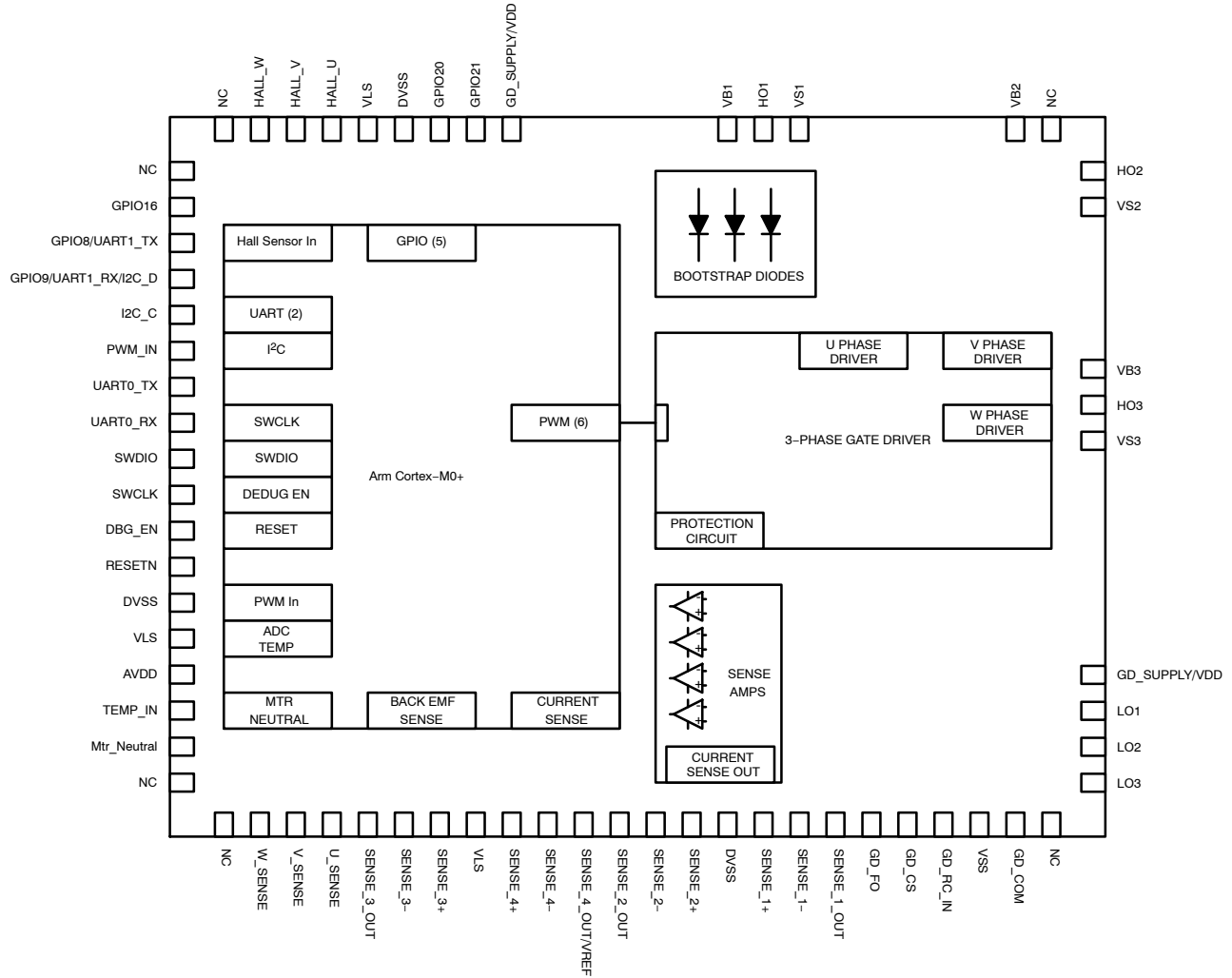
Figure 1. Block Diagram
