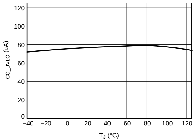
Figure 10. Current Consumption, V_{CCOFF} = 0.1 \text{ V} , V_{CS} = 0 \text{ V} , ver. D
