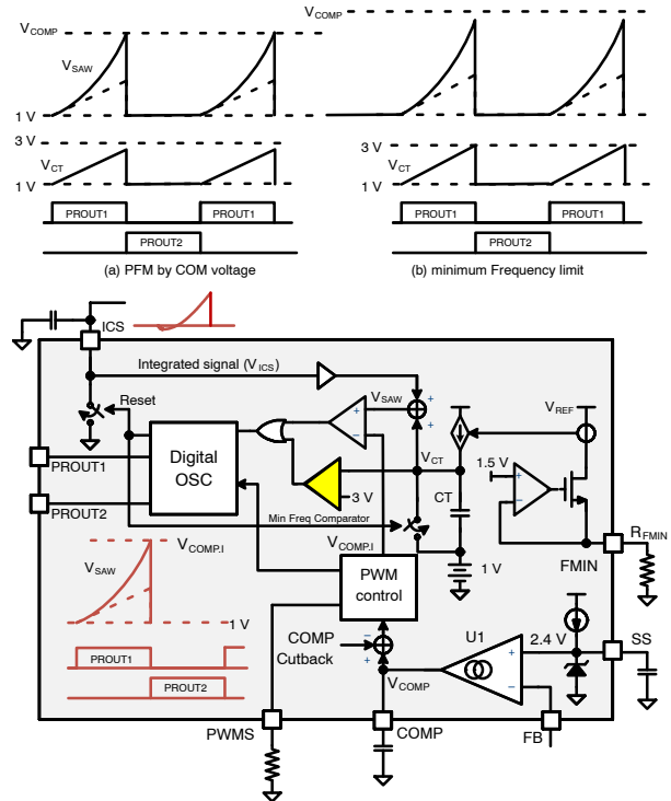
Figure 74. Minimum Switching Frequency Setting
