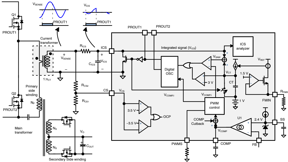
Figure 83. Basic Application Circuit for Current Sensing and Soft-Star
