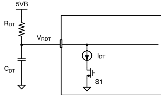
Figure 72. Internal Current Source for RDT Pin
