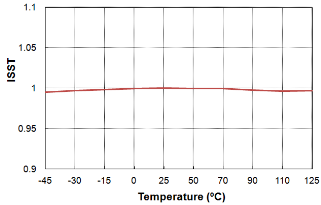
Figure 30. ISST vs. Temperature
