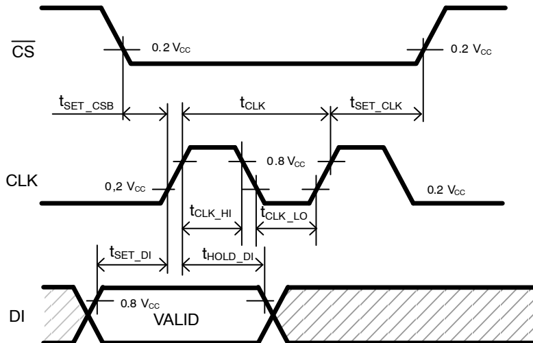
Figure 6. SPI Timing
