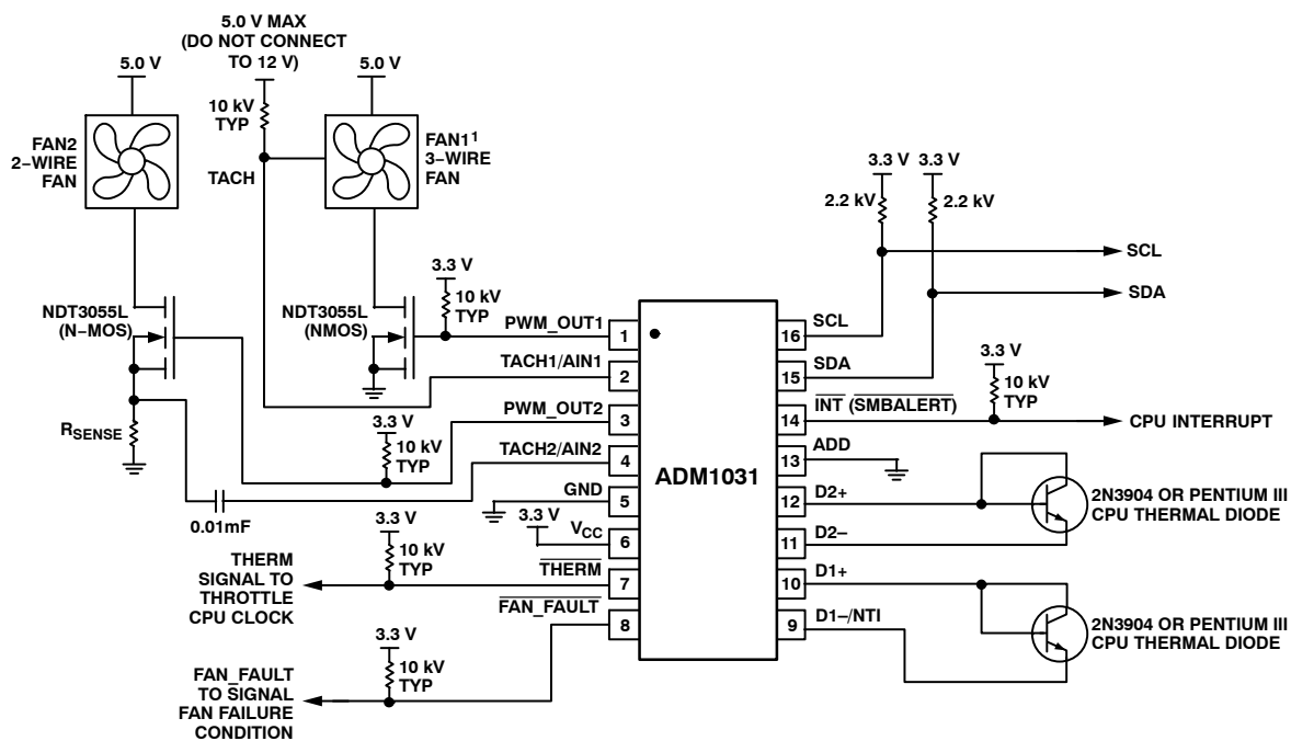
Figure 38. Operation of \overline{\text{FAN\_FAULT}} and Interrupt Pins
