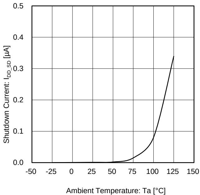
Figure 27. Shutdown Current vs Temperature ( V_S = 5\text{ V} )
