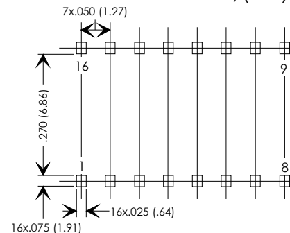
FIGURE 3: RECOMMENDED PCB LAYOUT DIMENSION IN INCHES, (mm)
