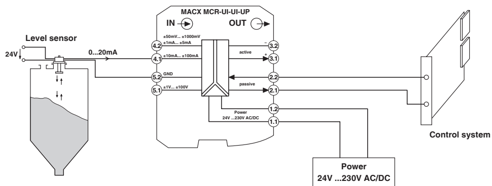
Application drawing
