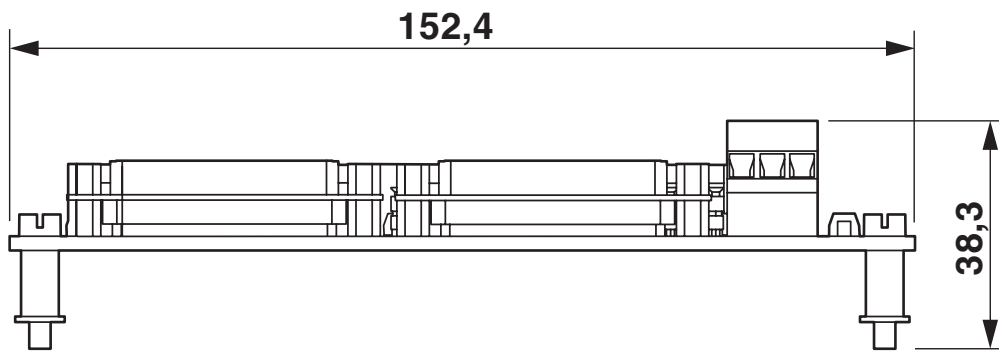
Dimensional drawing
