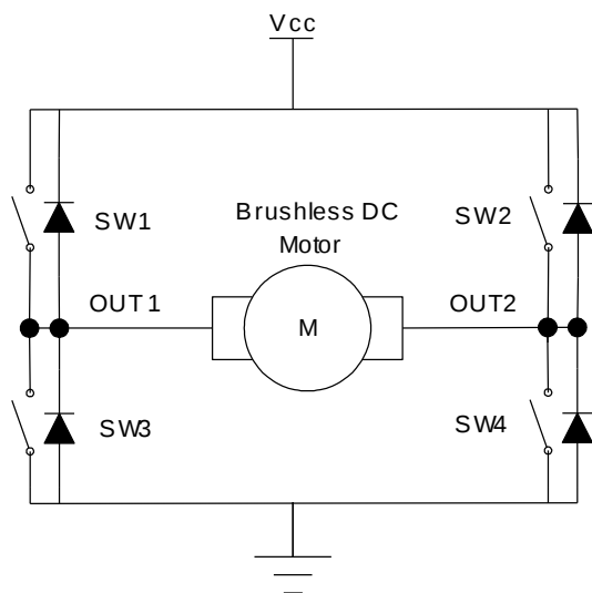
Figure 3: Power Stage
