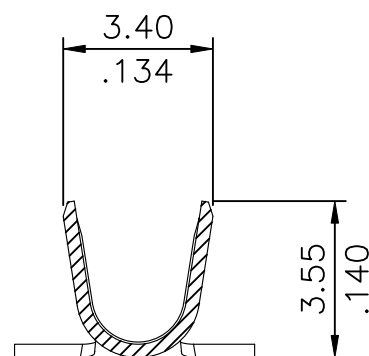
SEC. A-A (S: 4/1) P/N: CP60T03*PP0-HC
