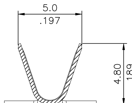
SEC. A-A (S: 4/1) P/N: CP60T04*PP0-HC
