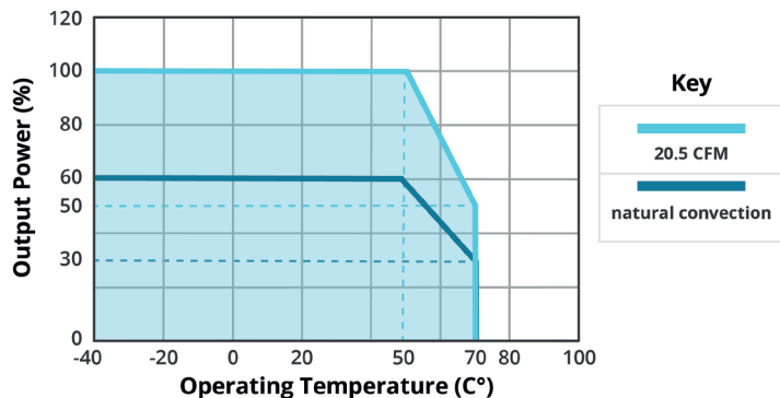
TEMPERATURE DERATING CURVE (full load 300W with 20.5 CFM) VMS-350C-12
