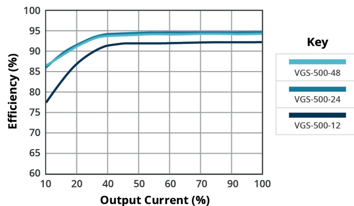
EFFICIENCY VS OUTPUT CURRENT (Vin = 230 Vac)
